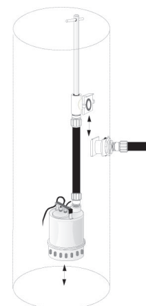
Enkeladaptermontage
