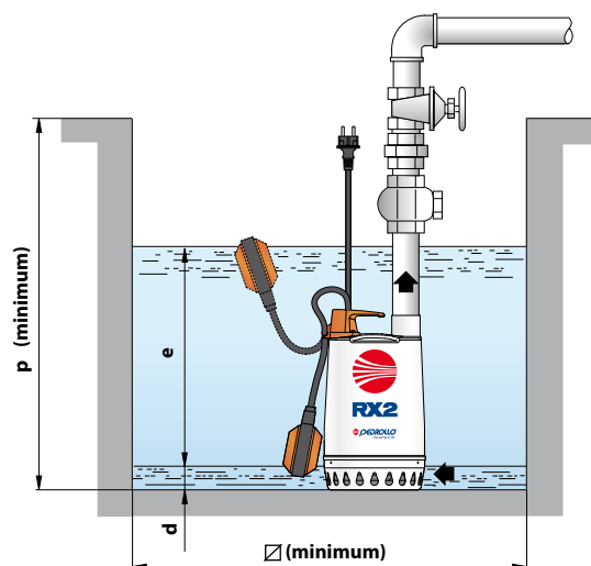
Typical installation
