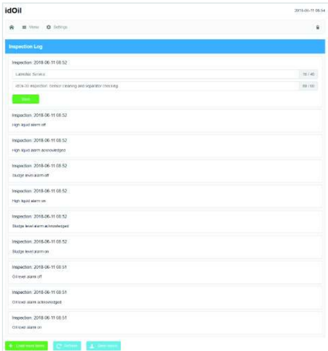
Figure 33. Inspection log
