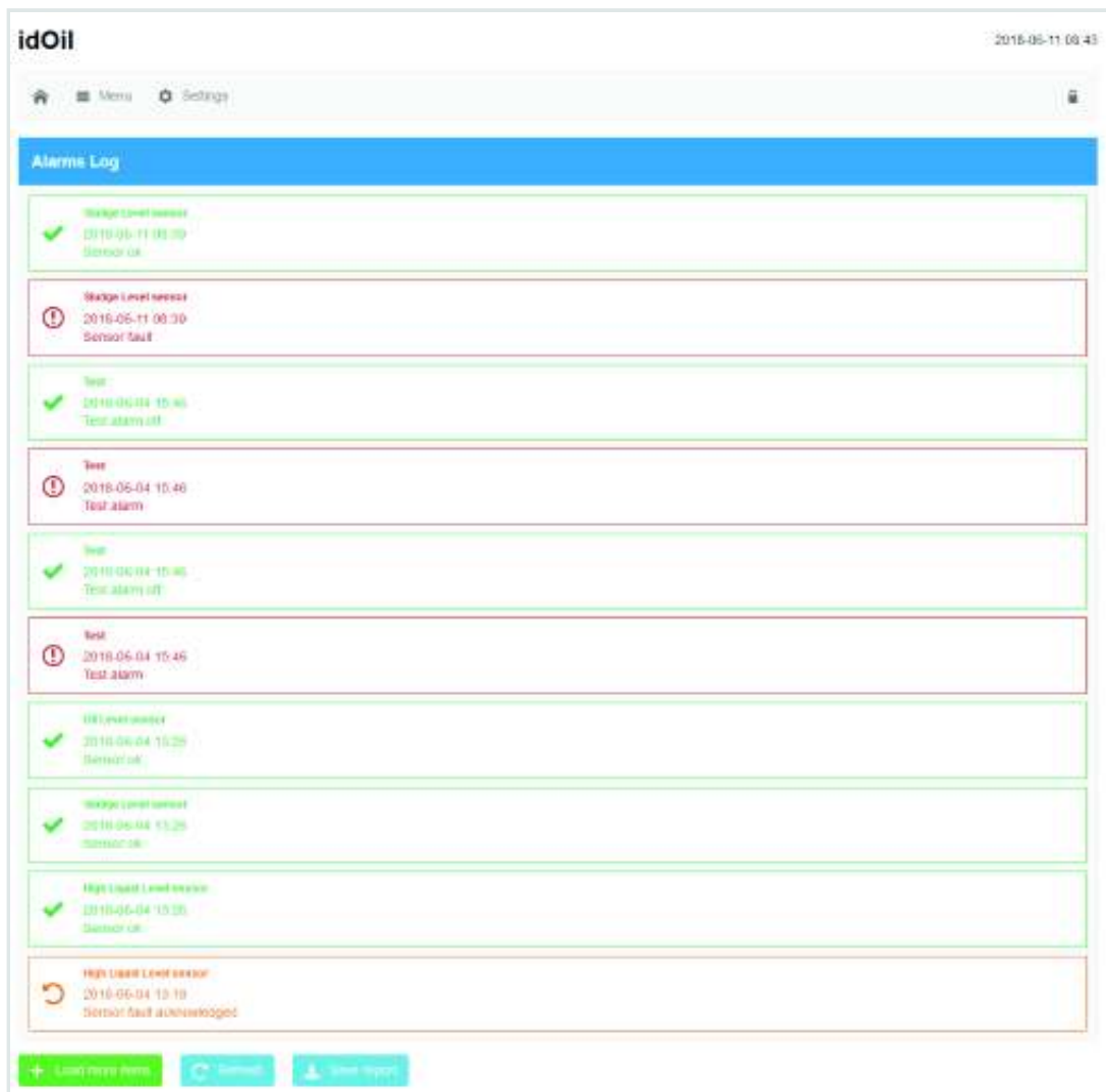
Figure 31. Alarm log
