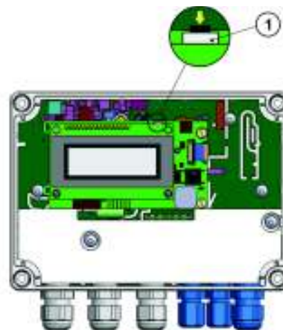
Figure 17. Sensor identification button.
