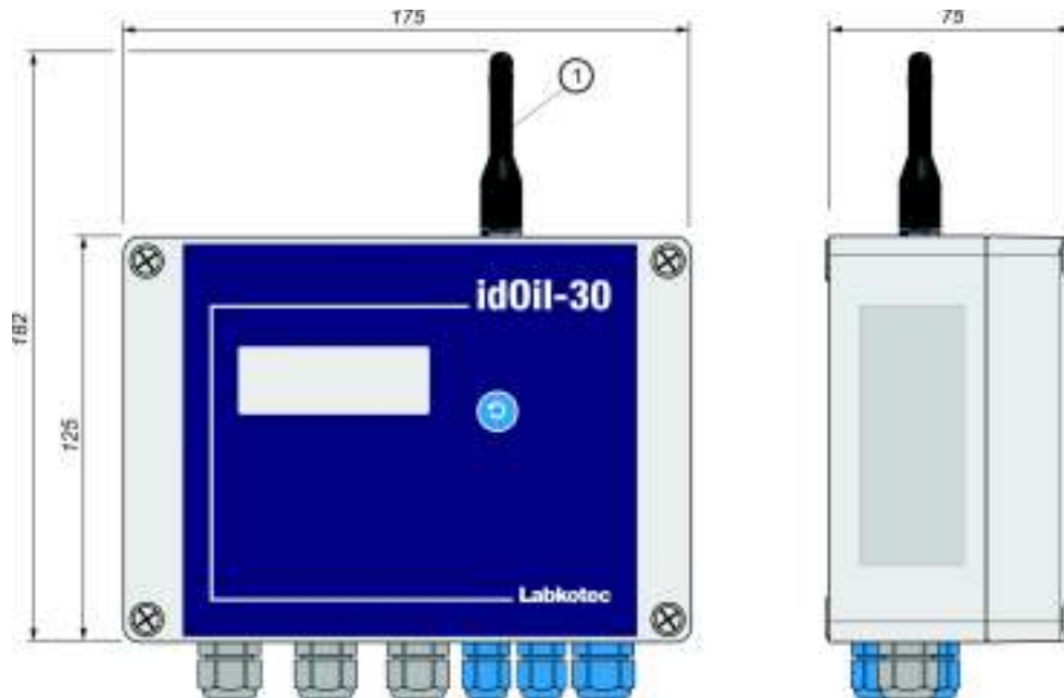
1 idOil-30 3G model with antenna (option)
