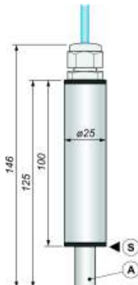
Figure 3. High liquid level sensor idOil-LIQ – structure and dimensions (mm)
