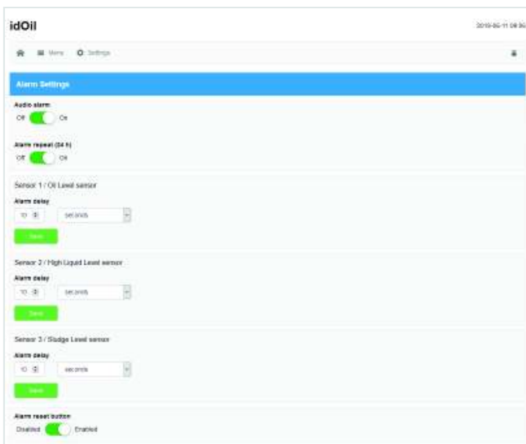
Figure 40. Alarm settings
